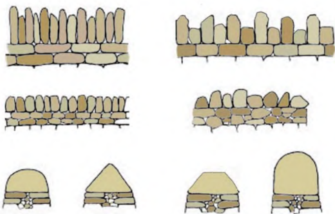
Stone coping details
